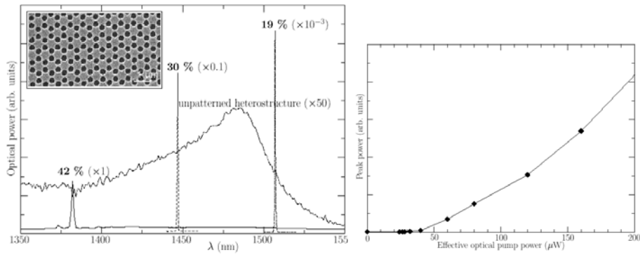
Figure 12: emission spectra of the surface emitting laser formed in a graphite lattice 2D PC, for different hole filling factors (f). The plot of the emitted power versus the pumping power indicates a threshold power of 40 \mu\text{W} for f = 19\% .
