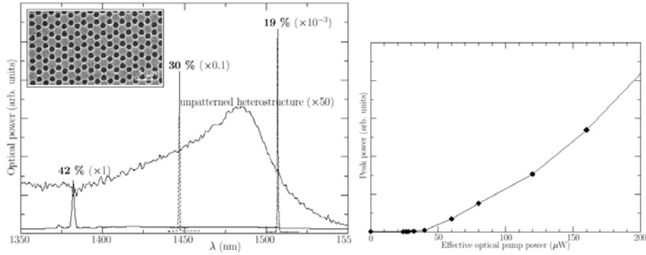
Figure 12: emission spectra of the surface emitting laser formed in a graphite lattice 2D PC, for different hole filling factors ( f ). The plot of the emitted power versus the pumping power indicates a threshold power of 40 \mu\text{W} for f = 19\% .
