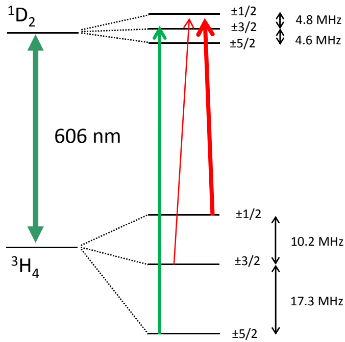
Figure 6: Three-level \Lambda -system in Pr^{3+} : Y_2SiO_5 . In addition to the two fields involved in the EIT process, a third beam is used to repump ions from the ^3H_4(\pm 5/2) ground state sublevel. Repumping serves to select the active ions within a narrow spectral interval, thus reducing the effective inhomogeneous width.
