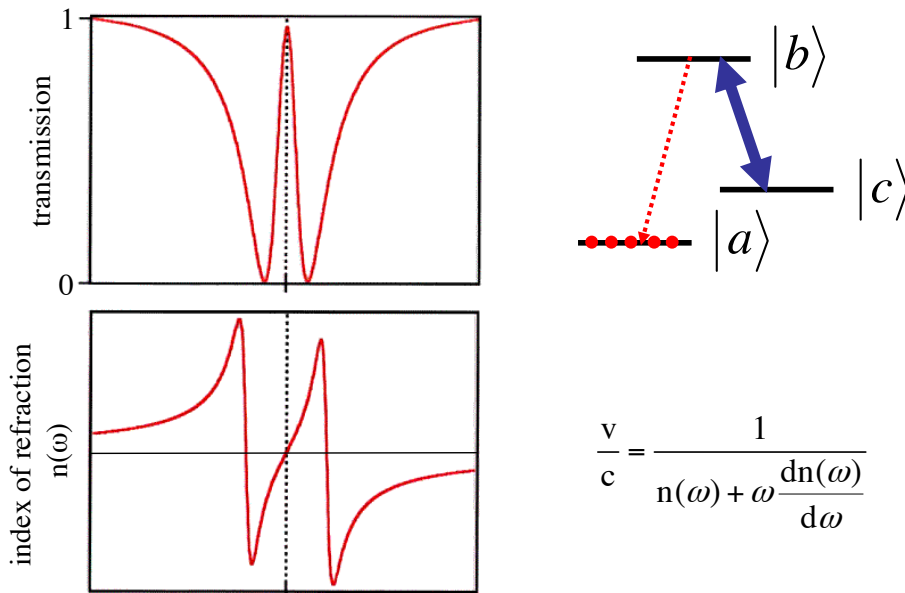
Figure 1: Principle of EIT. All atoms are initially prepared in state |a\rangle . The coupling field, resonant with the b \rightarrow c empty transition, opens a transparency window on the a \rightarrow b transition. The absorption profile distortion goes along with modified dispersion of the index of refraction. This is reflected in group velocity reduction within the transparency window.
