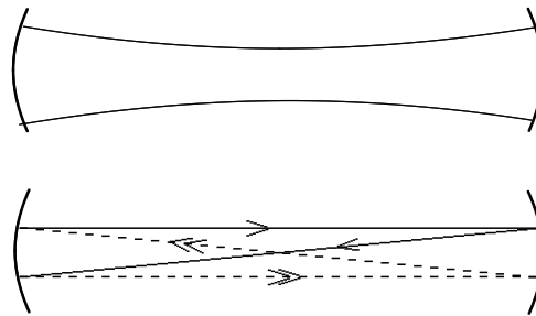
Figure 11 - Modes laser
